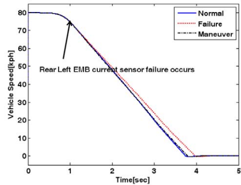
Fig. 9 Comparison of the vehicle speeds
