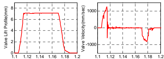
Fig. 11 Valve lift and velocity profile (Actual)
