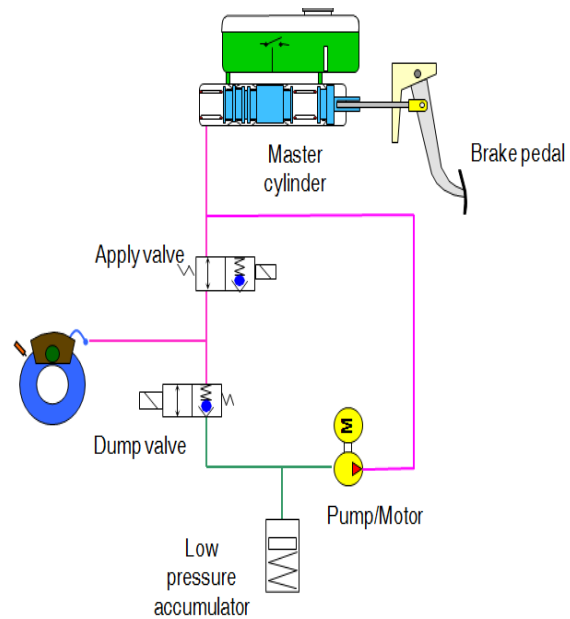
Fig. 2 ABS system diagram
